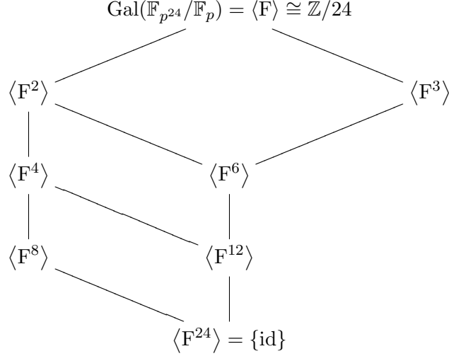
FIGURE 5.2. The subgroups of the Galois groups of \mathbb{F}_{p^{24}}/\mathbb{F}_p
