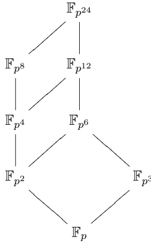
FIGURE 5.1. The subfields of \mathbb{F}_{p^{24}}
